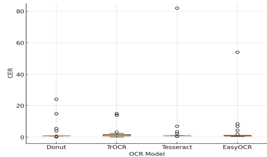
Fig. 13. CER Comparison of OCRs on the UM-PTI-Handwriting Dataset
